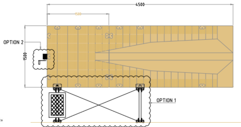
3 SEATER JETSKI DOCK SCALE 1:30
